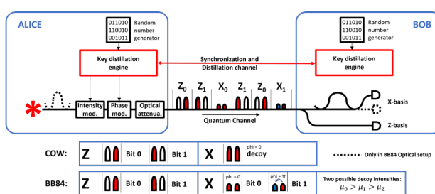
COW/BB84 optical schema
